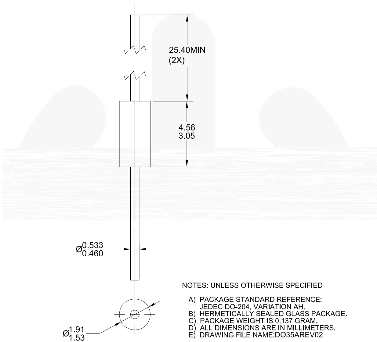
Figure 11. AXIAL LEADED, GLASS, JEDEC DO204, VARIATION AH, DO-204AH (DO-35)
